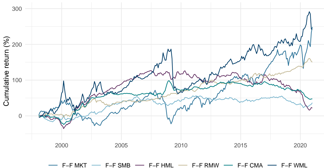
Figure 1 Cumulative returns, global Fama-French factors, 1998-2020
