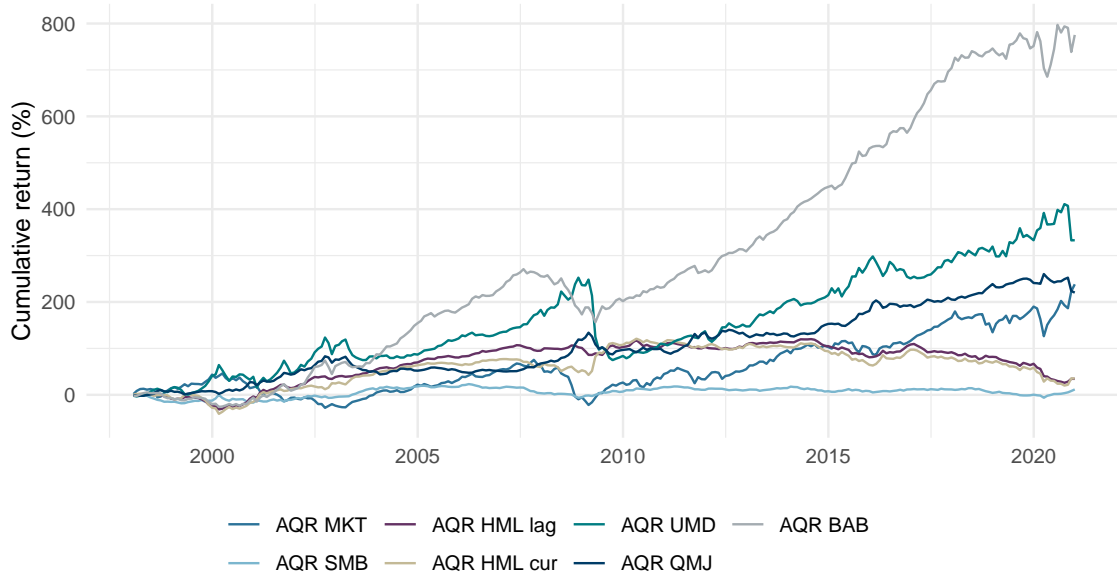
Figure 6 Cumulative returns, global AQR factors, 1998-2020
